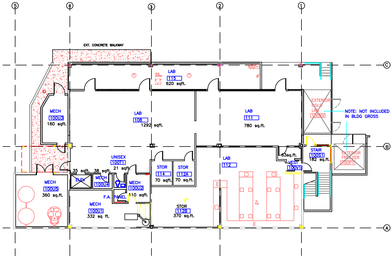
ANDERSON BUILDING – FIRST FLOOR Building No.: JS-109
